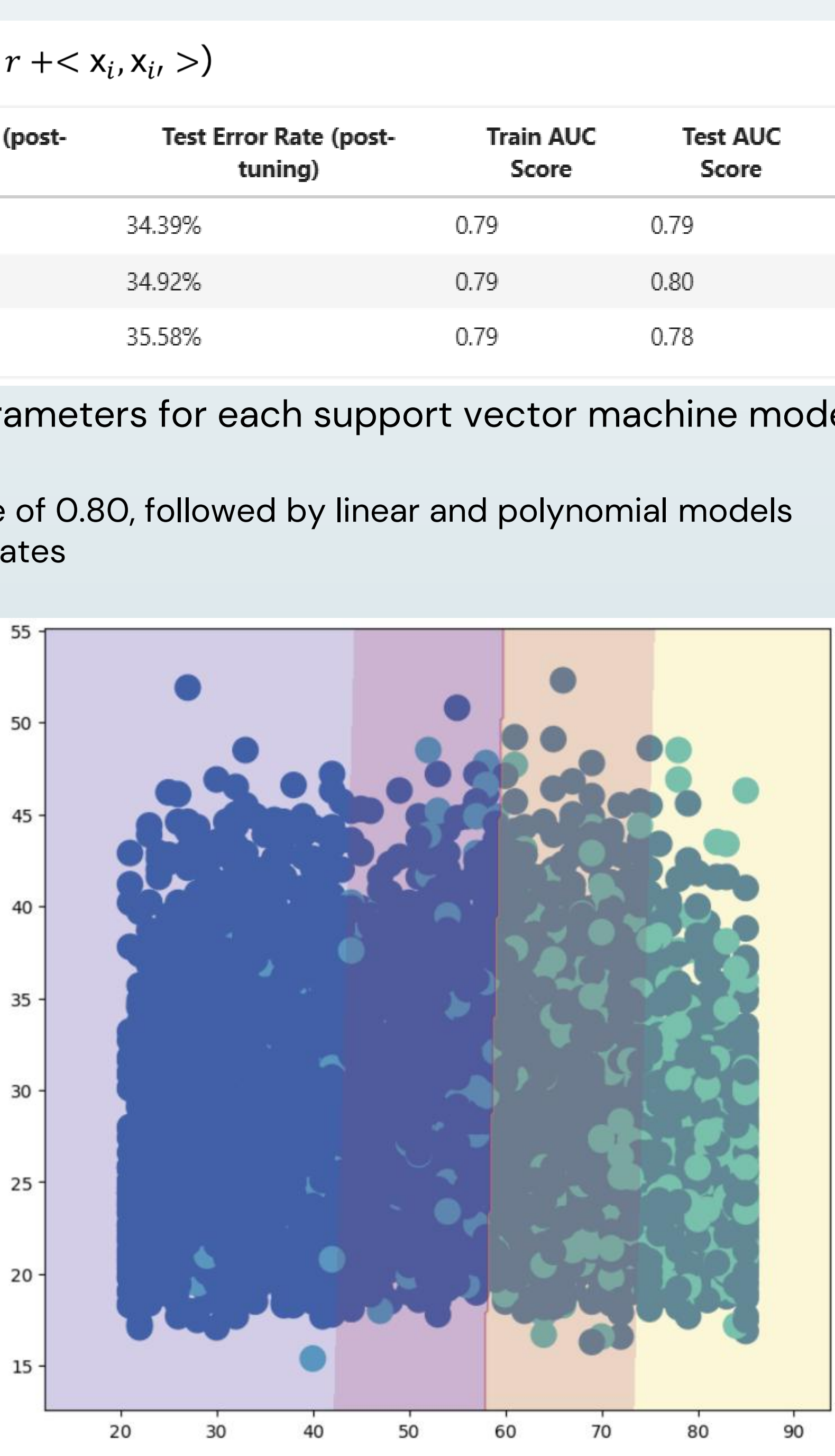
Figure 3. Linear decision boundary for linear kernel model comparing age (x-axis) and body mass index (y-axis)
